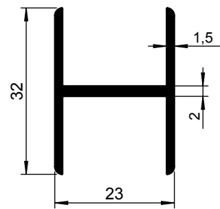
1256 095-000 1256 095-001 TZ
