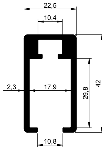
6296 345-000 7500 mm 6296 345-016 TZ 7500 mm
