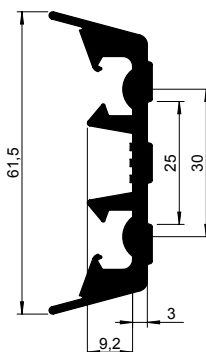
Stootrubber 55 mm 2460 055-000
