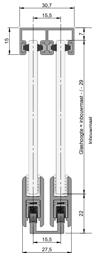
Aluminium glasrailsysteem 5-7 mm - 6303
